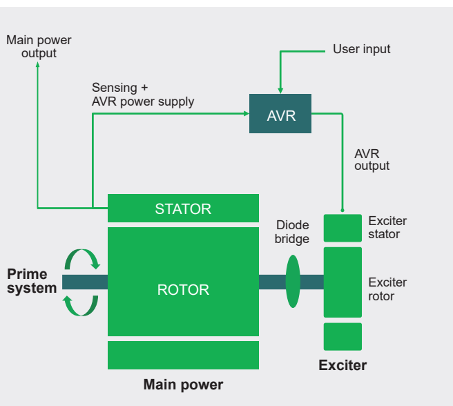
Diagram of a complete excitation system
